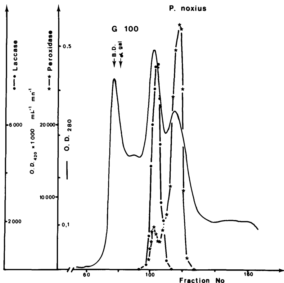
Fig. 4. Elution profile of total proteins and laccase and peroxidase activities on Sephadex G-100. The most laccase-active fractions collected after the DEAE-cellulose chromatography shown in Fig. 3 were chromatographed.
