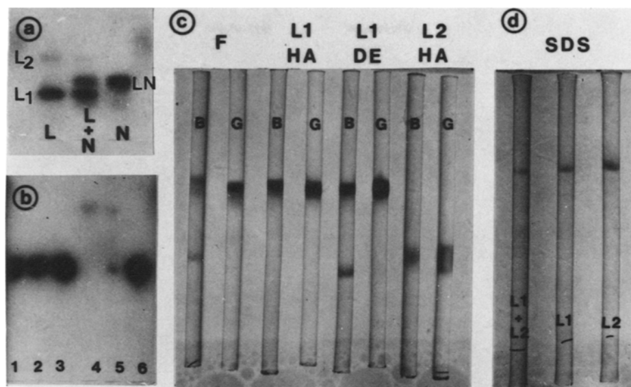
Fig. 1. (a) Laccase isozyme pattern after starch gel electrophoresis of crude culture filtrates from R. lignosus (L) and P. noxius (N); (L + N = mixture (v/v) of the two types of culture filtrates); L1 and L2 are the two laccase isoenzymes corresponding to the isoenzymes shown in Fig. 2. (b) Control of L1 and L2 at different purification steps: 1, 2, and 3, L1 fractions eluted from the hydroxylapatite (HA) column; 4, L2 after the HA step; 5 and 6, respectively, L2 and L1 after the DEAE-cellulose chromatography step. (c) L1 and L2 purity control (polyacrylamide gel electrophoresis): B, Coomassie blue staining; G, laccase activity. Protein and laccase patterns: F, crude culture filtrate; L1HA and L2HA, L1 and L2 fractions after the HA chromatography step; L1DE, L1 fraction after the DEAE-cellulose chromatography step. (d) Proteinogram of the purified laccases L1 and L2 under denaturing conditions (SDS).
