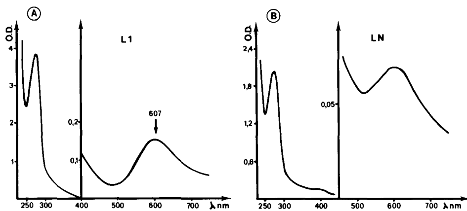
Fig. 5. Spectral characteristics of R. lignosus L1 (A) and P. noxius LN (B) laccases.
