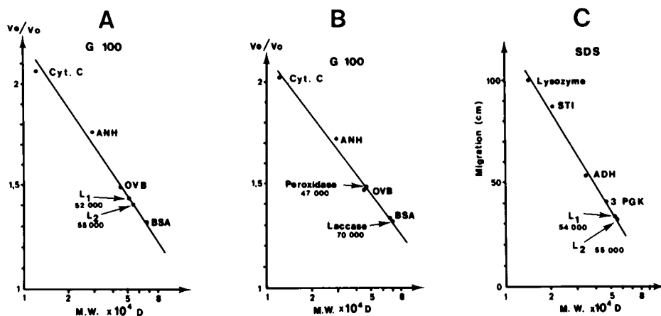
Fig. 6. Molecular weight estimation of R. lignosus L1 and L2 laccases (A) and the P. noxius enzyme (B) under nondenaturing conditions. These determinations were performed with the Sephadex gel filtration method. (C) MW determination (SDS-polyacrylamide gel electrophoresis) of L1 and L2 under denaturing conditions. Previous to the electrophoresis, the proteins were denaturated by incubation for 10 min at 100°C in a Tris-HCl 0.2M, pH 8.5, buffer, containing 1% SDS.
