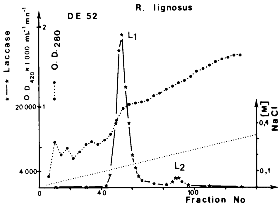
Fig. 2. Elution profile of the proteins (as OD_{280nm} ) and laccases L1 and L2 on DEAE-cellulose. NaCl gradient: 0–0.35M in a Tris-HCl 0.025M, pH 8.4 buffer; total vol, 700 mL; fraction vol, 5 mL; elution speed, 60 mL/h.
